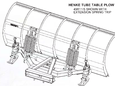
▲ Henke Tube Table and A Frame Assembly
